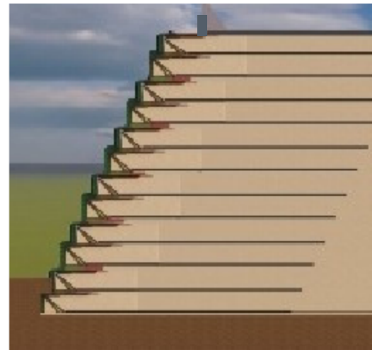
WELDED WIRE FACED REINFORCED SLOPES & WALLS
