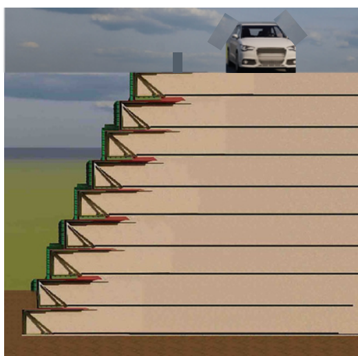
TEMPORARY SHORING - STAGED CONSTRUCTION
